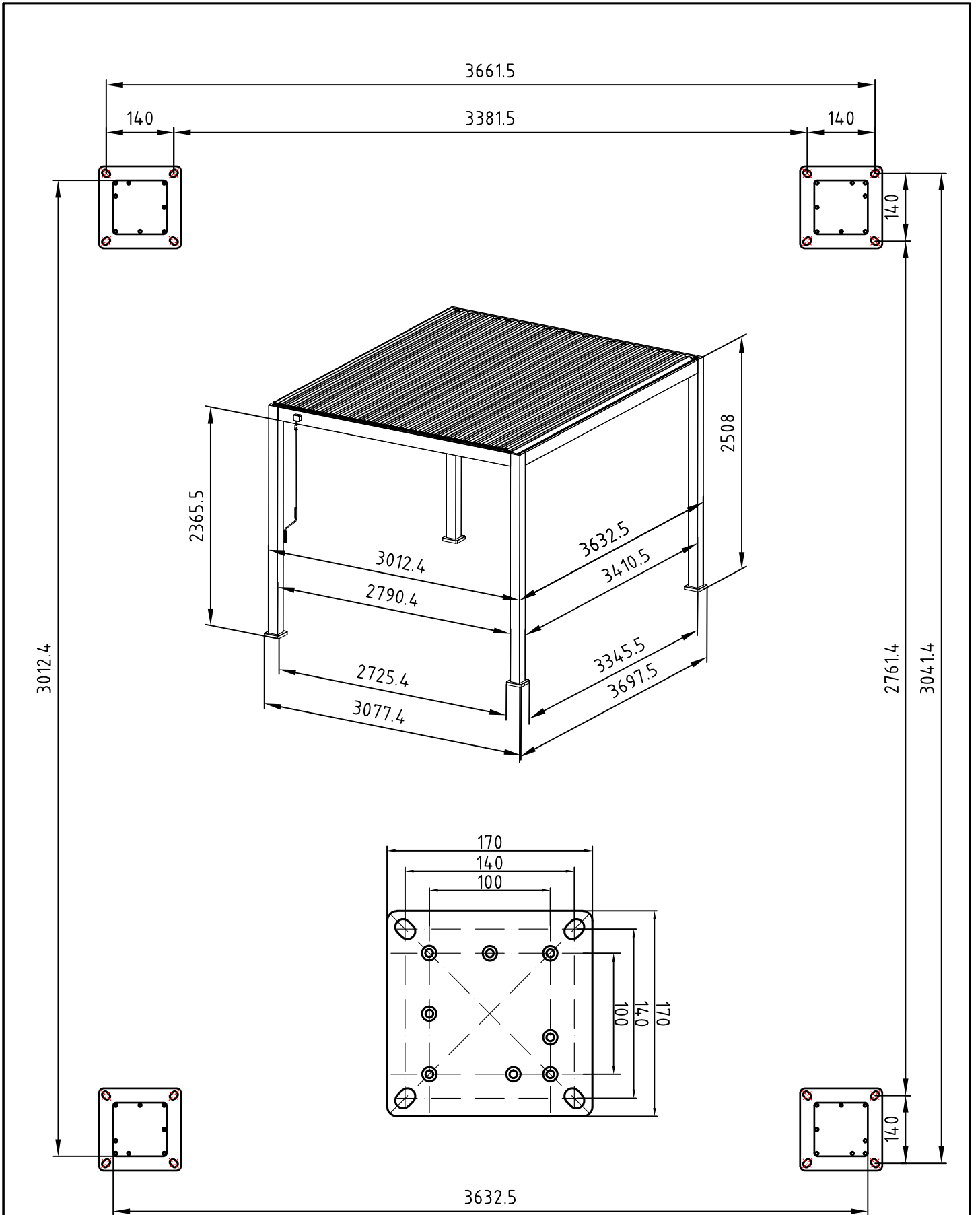
Alvaro gazebo 360x300x250
